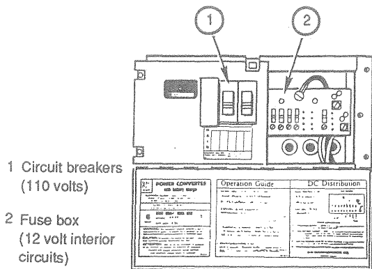
Typical Power Converter
