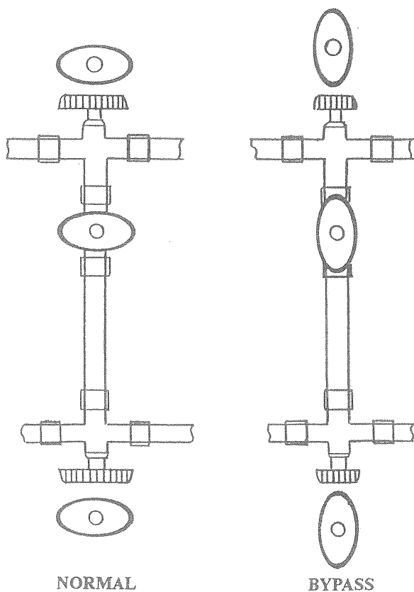
Water Heater Bypass Valves
