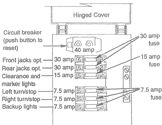
Exterior Light Fuse Box
